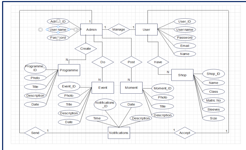
Figure 4.2 Entity Relationship Diagram
