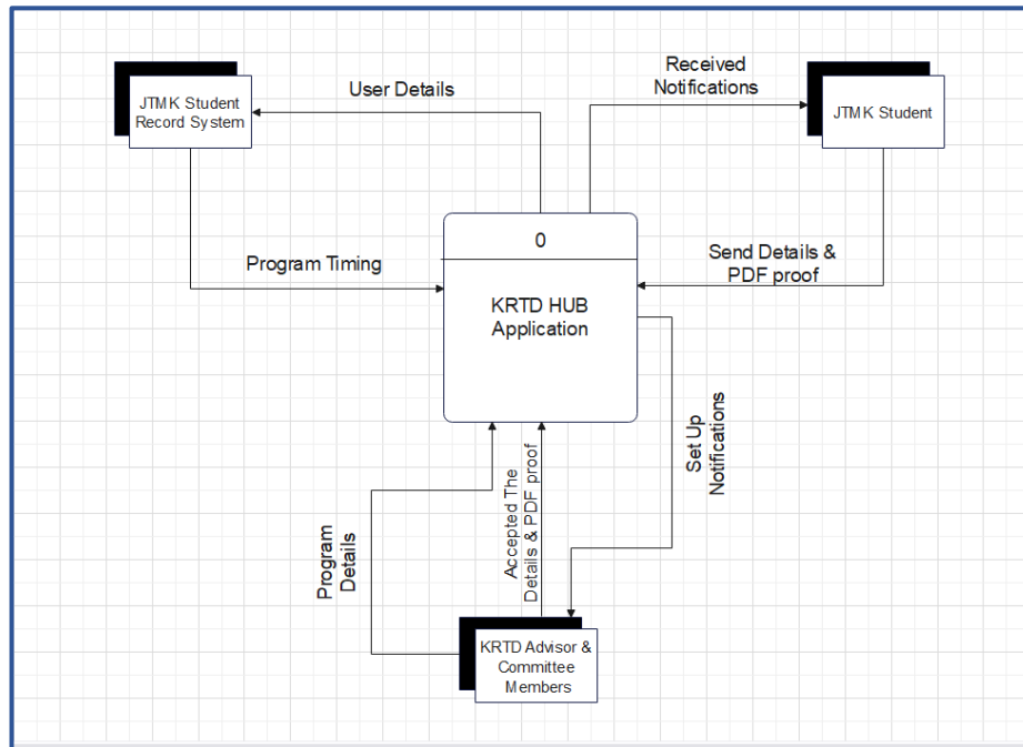
Figure 4.0 Data Flow Diagram : Context Diagram
