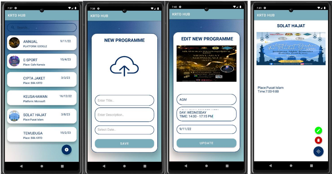
Figure 6.5 Our Programme Admin Page Interface
